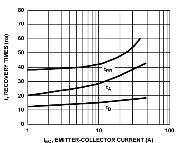
FIGURE 14. TYPICAL tRR, tA, tB vs FORWARD CURRENT
