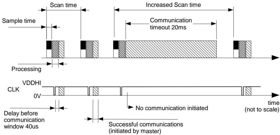
Figure 6-2 How to use RDY signal on clock line
