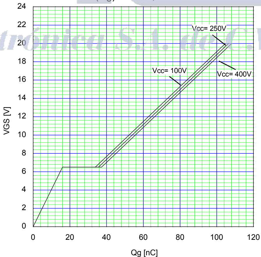
Typical Gate Charge Characteristics V GS =f(Q g ):I D =21A,T ch =25°C
