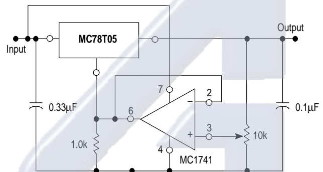
Figure 15. Adjustable Output Regulator
