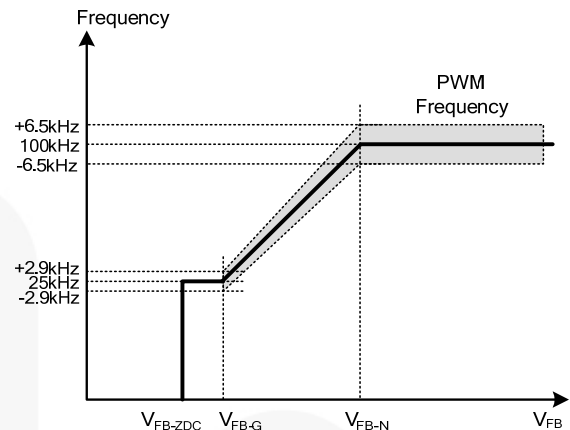
Figure 23. PWM Frequency
