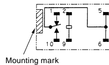
Terminal arrangement/ Internal connections (bottom view)
