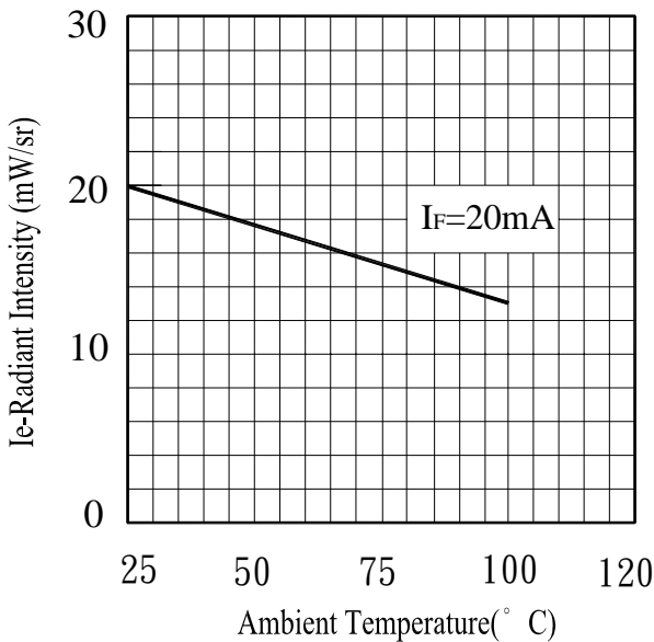
Fig.7 Radiant Intensity vs. Ambient Temperature( ^\circ\text{C} )
